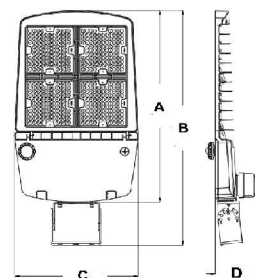
Trunnion mount
