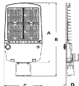
Dimensions Trunnion Mount 51L
