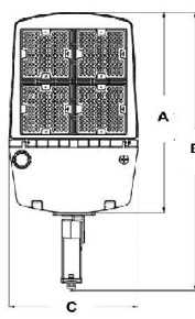
Dimensions Slip fitter 51L
